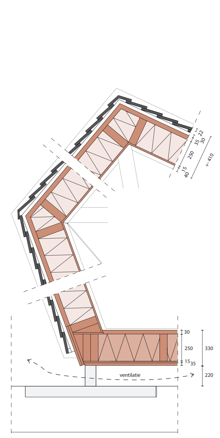
Detail 1:20
